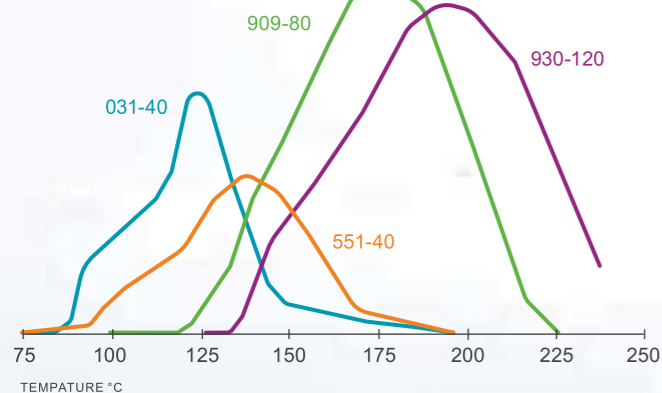
Expansion curves for several Expancel products
